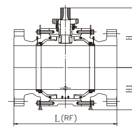
Internal supporting structure
