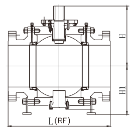
External supporting structure
