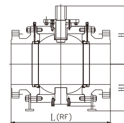
External supporting structure
