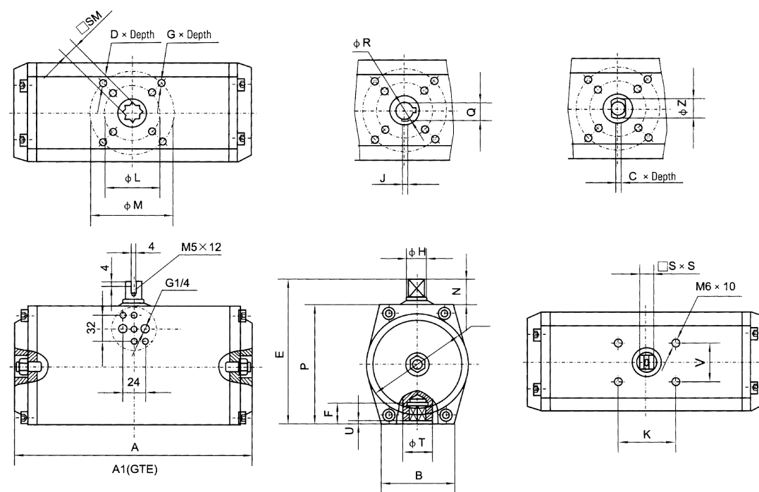
Outline and connection dimensions
