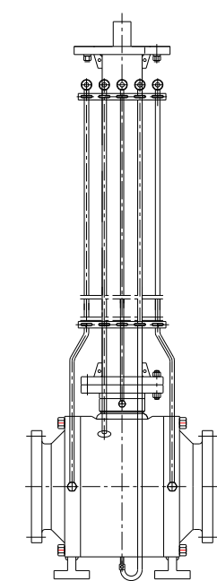
Schematic diagram of extension stem
